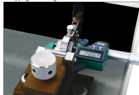
lapping measuring surfaces of outside micrometer
